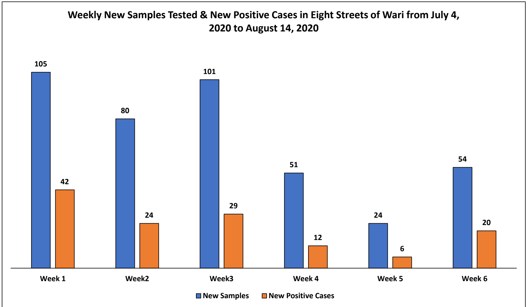
Figure 2: Weekly New Samples Tested & New Cases Detected in Eight Streets of Wari from July 4, 2020 to August 14, 2020
