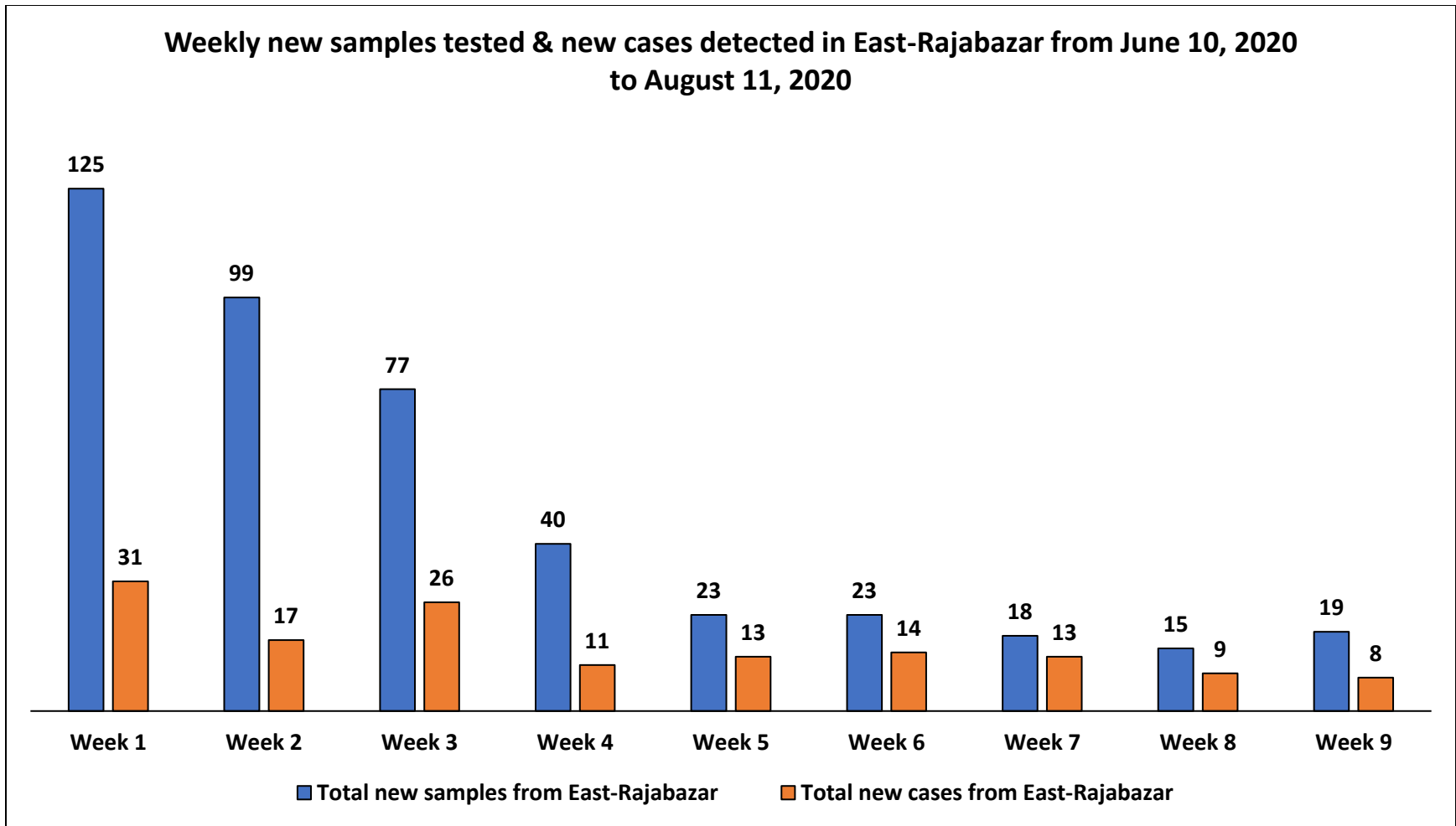
Figure 2: Weekly new samples tested & new cases detected in East-Rajabazar from June 10, 2020 to August 11, 2020
