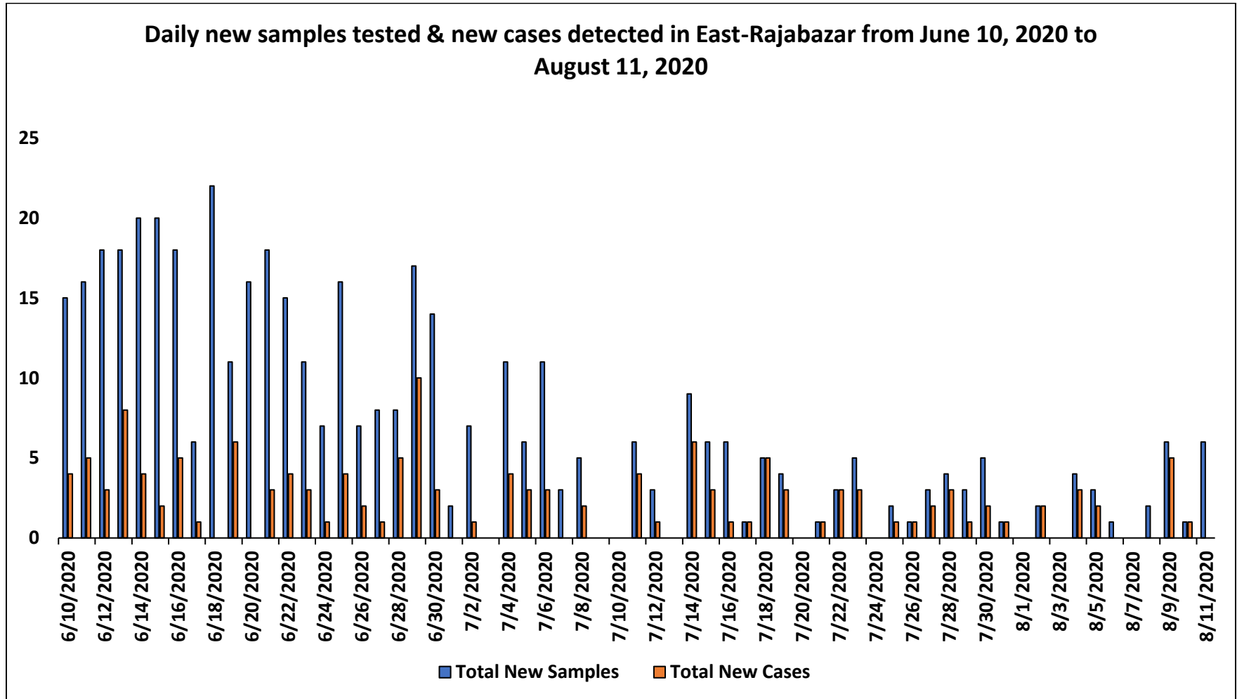
Figure 1: Daily new samples tested & new cases detected in East-Rajabazar from June 10, 2020 to August 11, 2020
