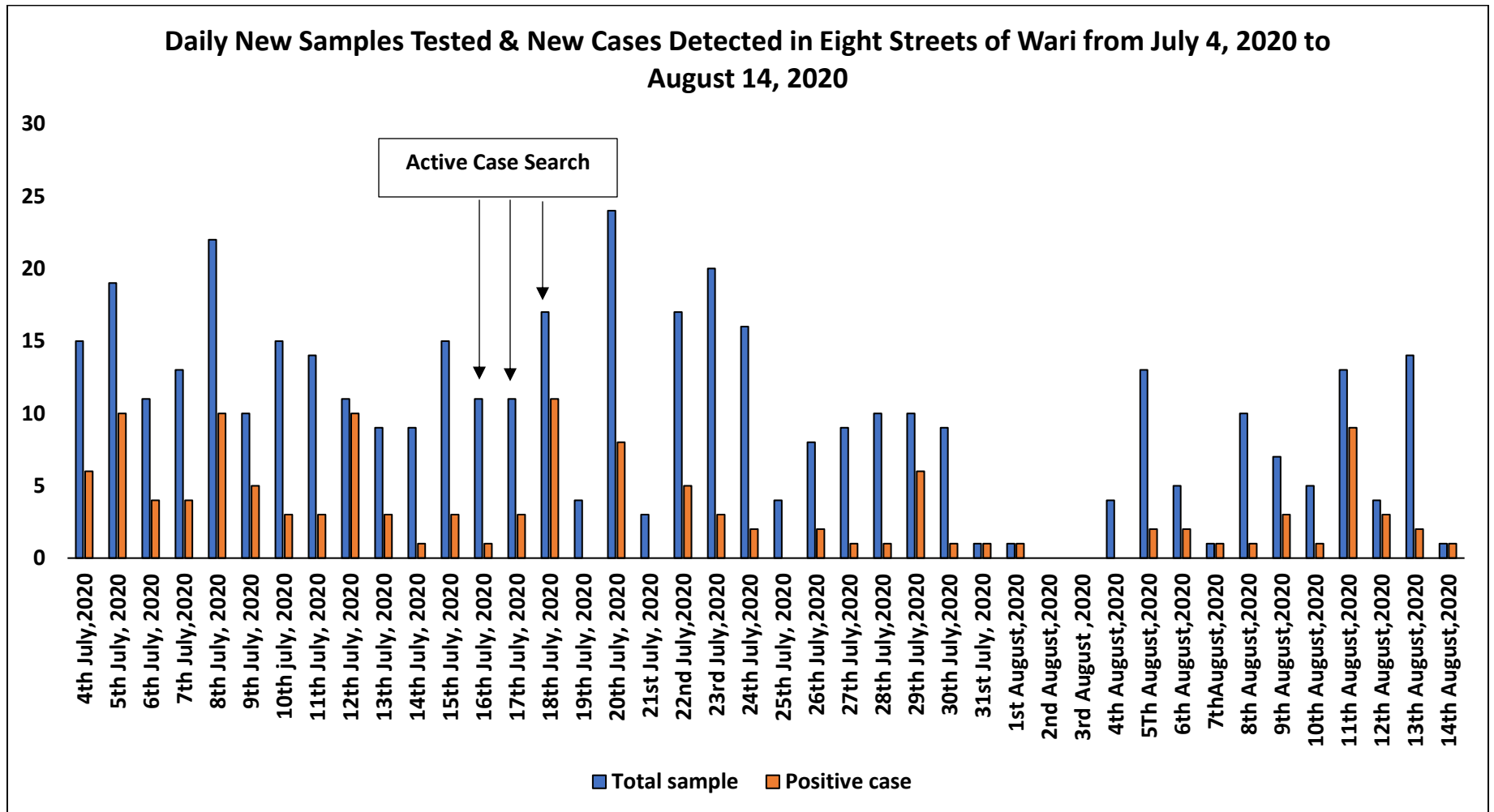
Figure 1: Daily New Samples Tested & New Cases Detected in Eight Streets of Wari from July 4, 2020 to August 14, 2020
